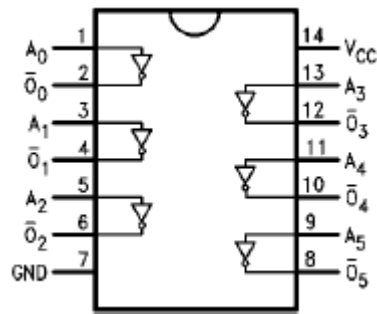
74AC04
