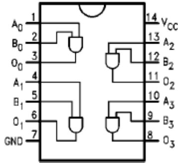
74AC08
