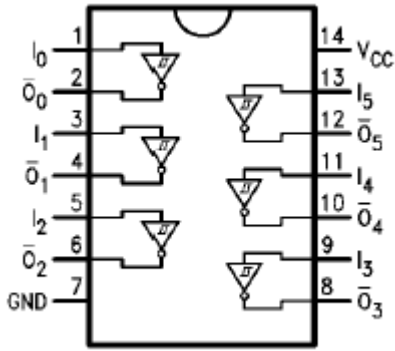
74AC14
