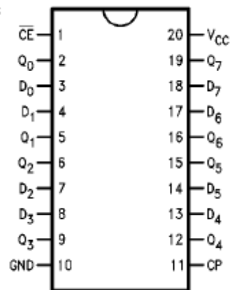
74AC377
